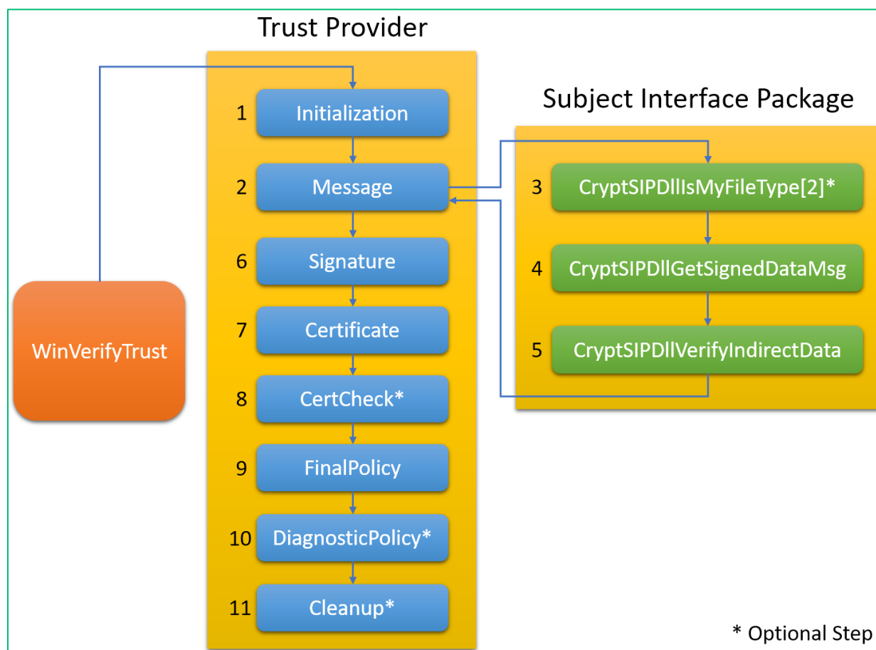
Illustration of the interplay between WinVerifyTrust, trust providers, and subject interface packages
