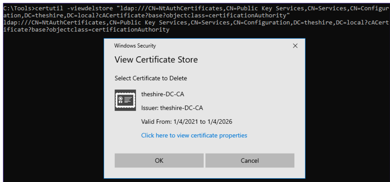
Figure 82 - Deleting Certificates from the NTAUTH store with certutil.exe
