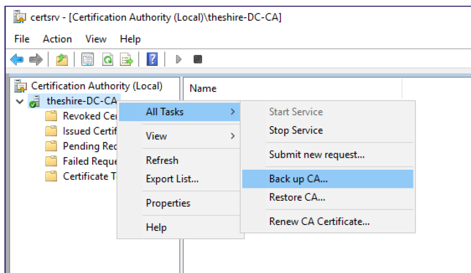
Figure 67 - Stealing CA Certificate Using certsrv.msc's Backup Functionality
